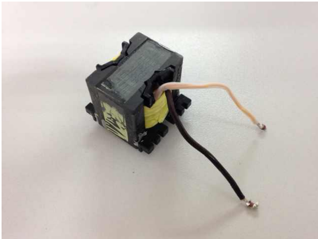
Picture 8: Internal view of transformer
