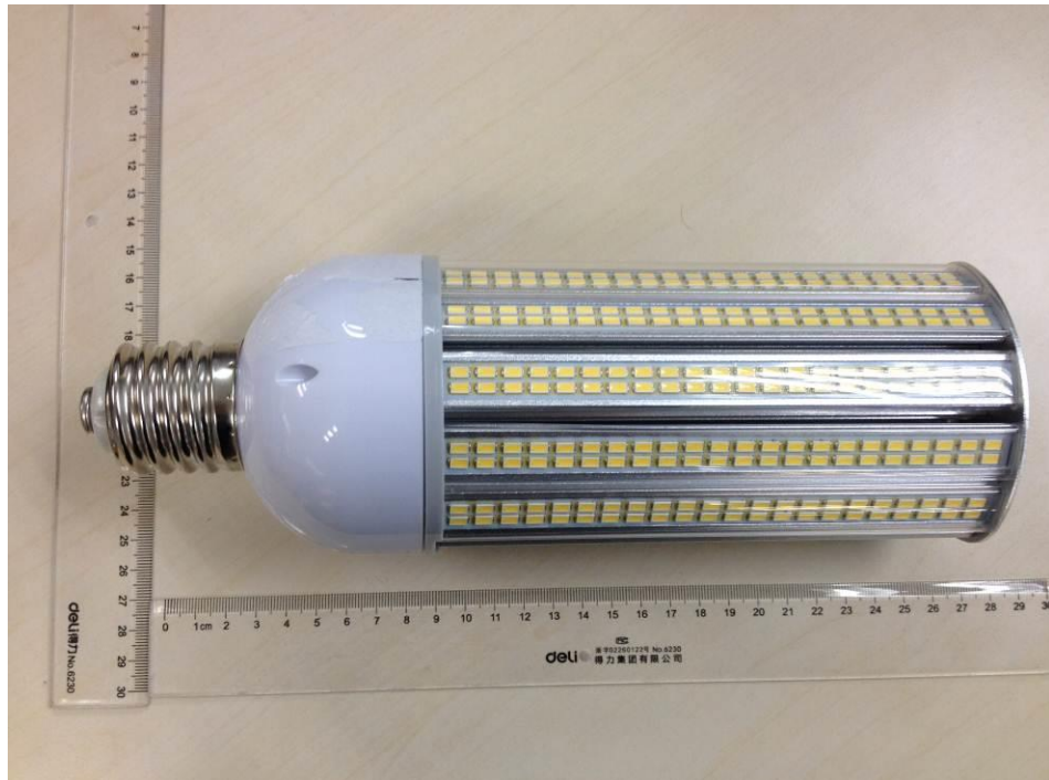
Picture 1: Overview of GKS13-40W (Others have different length)
