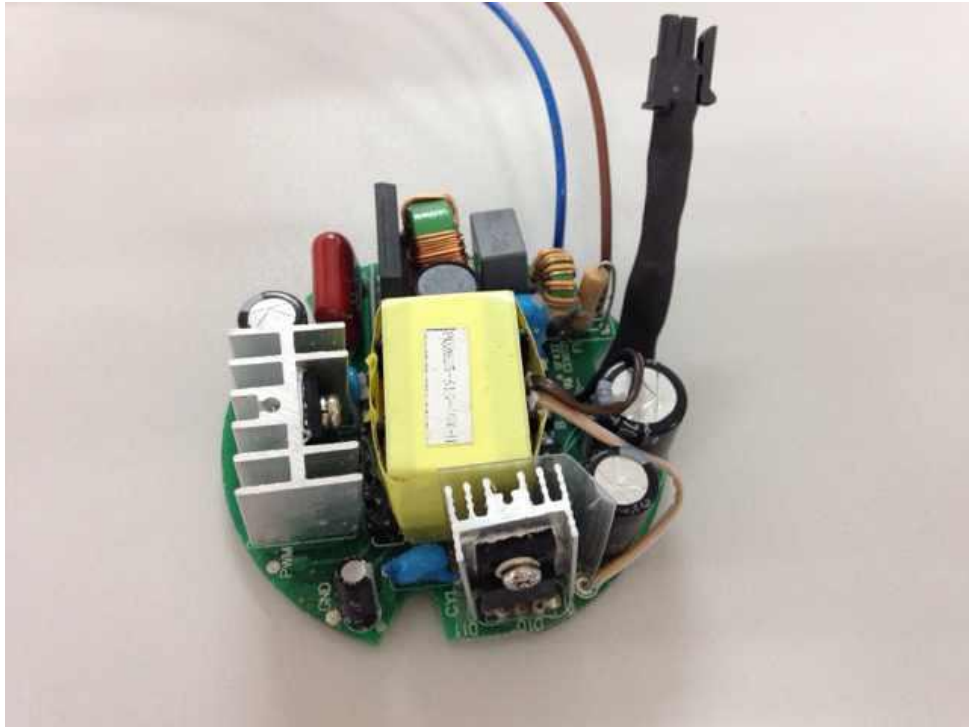
Picture 5: Top view of PCB
